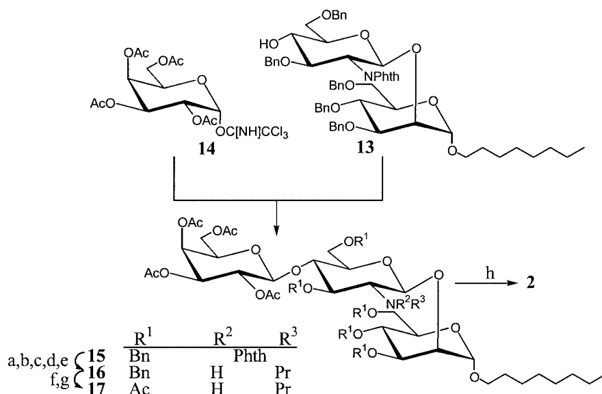
Scheme 2. Synthesis of trisaccharide 2 : a) NaOMe (pH = 9), CH 2 Cl 2 , MeOH; b) NH 2 CH 2 CH 2 NH 2 , 90 °C, 1-BuOH, molecular sieves (3 A); c) Pr 2 O, pyridine; d) NaOMe (pH = 9), MeOH; e) Ac 2 O, pyridine, 72% over five steps; f) 10% Pd/C, H 2 , HOAc, EtOH, EtOAc; g) Ac 2 O, pyridine, 65% over two steps; h) NaOMe (pH = 9), CH 2 Cl 2 , MeOH, 94%
